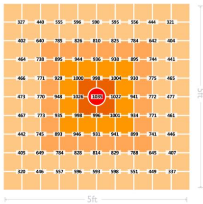
5ft*5ft grow tent, height 12" Previous generation product Avg PPF: 700 \mu\text{mol}/\text{m}^2/\text{s} ; Uniformity U1: 31%
