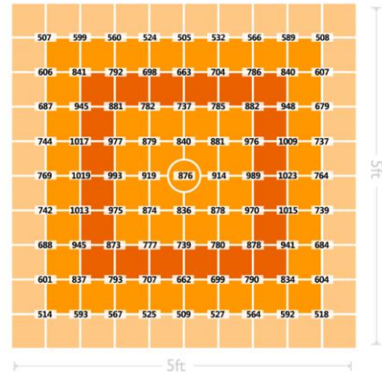
5ft*5ft grow tent, height 12" H series, Avg PPF: 757 \mu\text{mol}/\text{m}^2/\text{s} ; Uniformity U1: 50%
